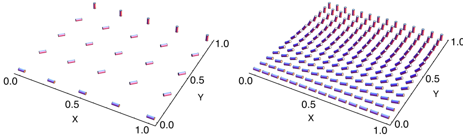
Fig. 4.2: Initial guess (left) on 4 \times 4 mesh with initial free energy of 12.534 and resolved solution (right) on 128 \times 128 (mesh restricted for visualization) with final free energy of 1.480 for a twist boundary.
